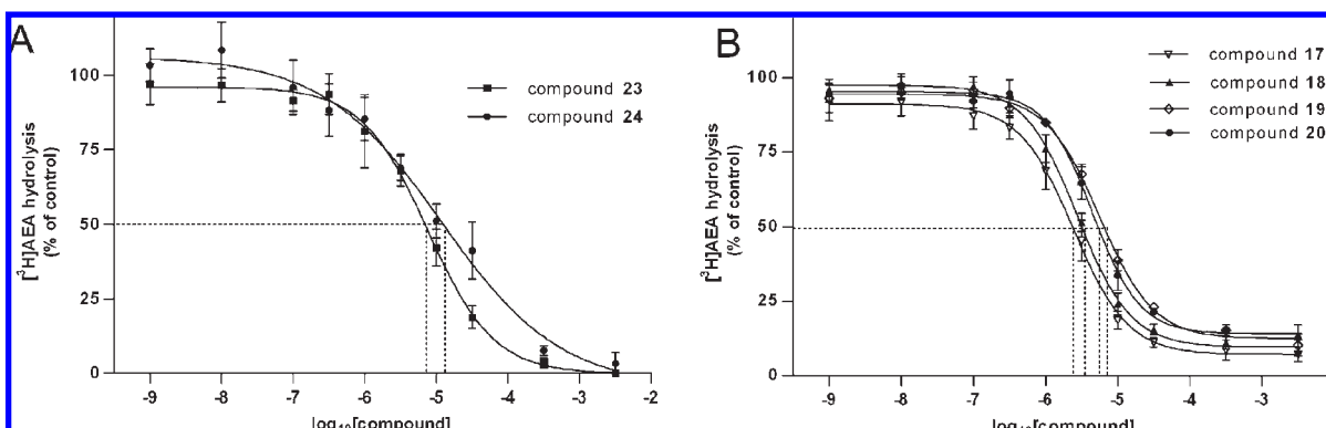
Figure 2. Inhibition of the hydrolysis by recombinant rat FAAH of 2 \mu\text{M} [ ^3\text{H} ]-AEA by compounds 23 and 24 (A) and compounds 17 , 18 , 19 , and 20 (B). Shown are means of three experiments, with no preincubation of the compounds with rFAAH prior to addition of [ ^3\text{H} ]-AEA. pIC 50 values are shown as a dotted line on the figure.
